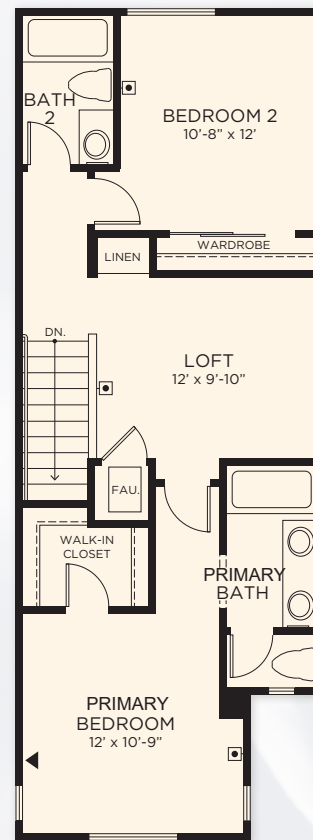
Second Floor
